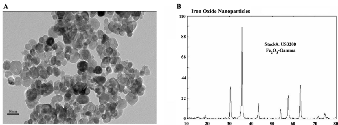
Figure 2. A: TEM electron micrograph of Fe_2O_3 nanoparticles, B: X-ray diffraction pattern (XRD) of Fe_2O_3 nanoparticles shows the structure. Initial peaks are indicating polycrystalline structure. Similarly, the secondary peaks are indicating the form of nanocomposites
